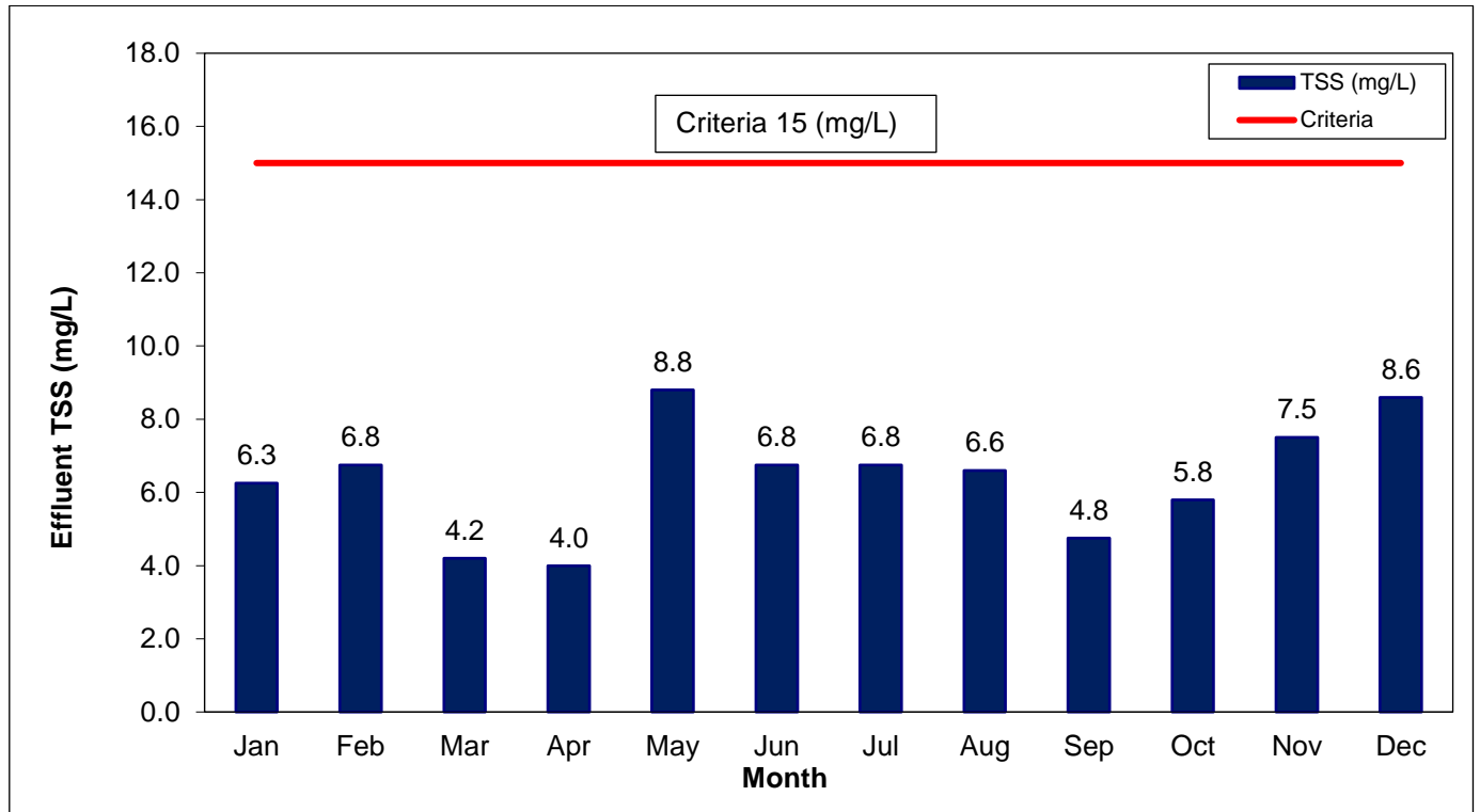
Ingersoll WWTP Effluent, Monthly Average TSS (mg/L), 2023
