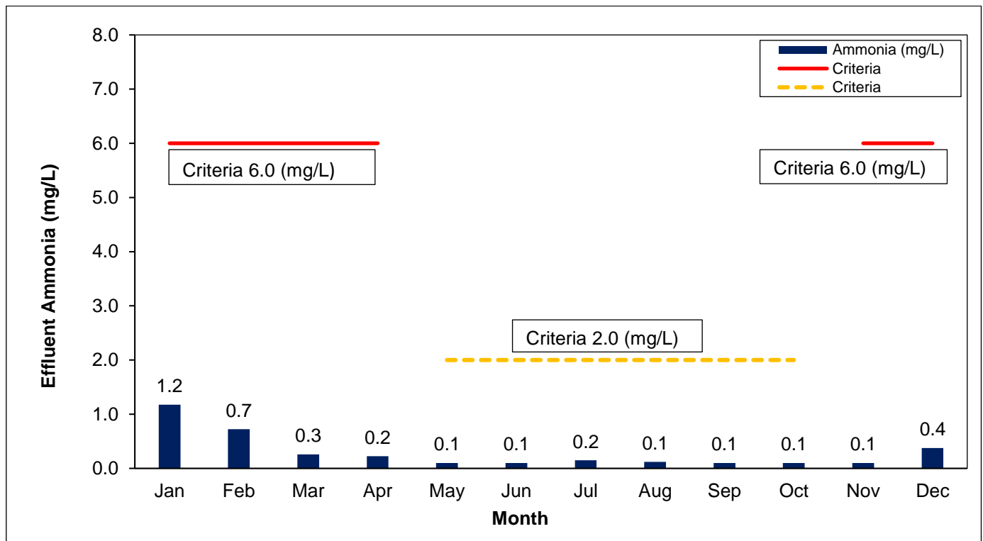
Ingersoll WWTP Effluent, Monthly Average Ammonia (mg/L), 2023
