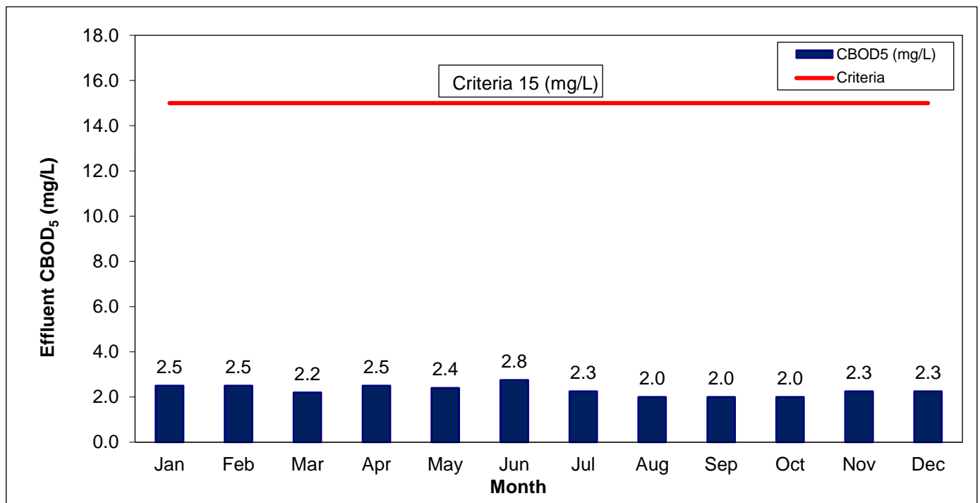
Ingersoll WWTP Effluent, Monthly Average CBOD 5 (mg/L), 2023
