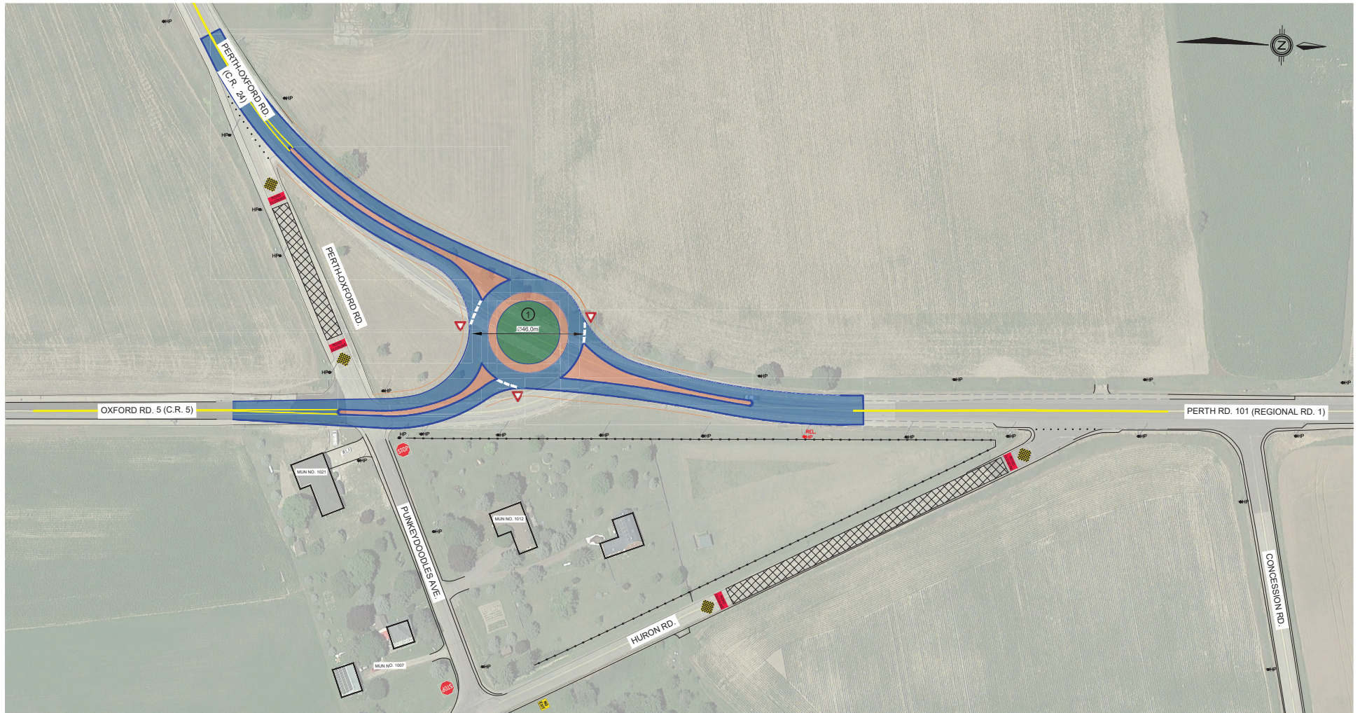
POTENTIAL LONG-TERM IMPROVEMENT ALTERNATIVES CONCEPTUAL ROUNDABOUT DESIGN OPTION #1
